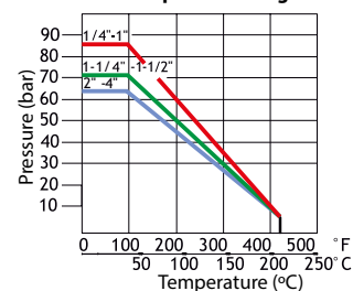
Pressure-Temperature Diagram
